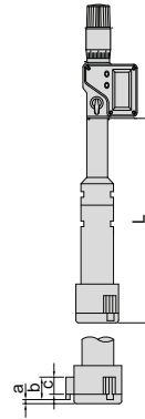
Type B 12-50mm, carbide measuring points
