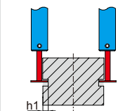
measuring external groove diameter ( h1 \leq 3.5\text{mm} )
