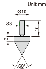
conical points (stainless steel)
