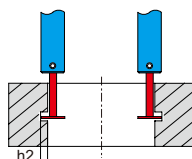
measuring internal groove diameter ( h2 \leq 3.5\text{mm} )
