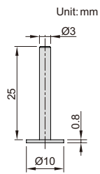
disk points (stainless steel)
